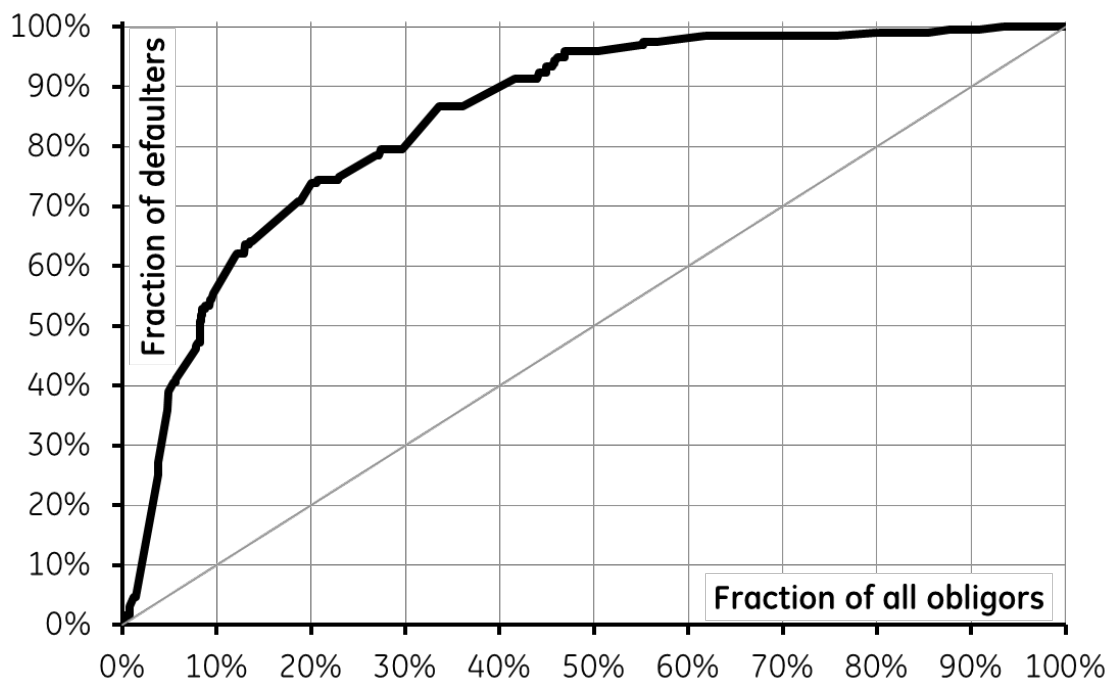
Figure 7. The ROC curve showing discriminatory power.
